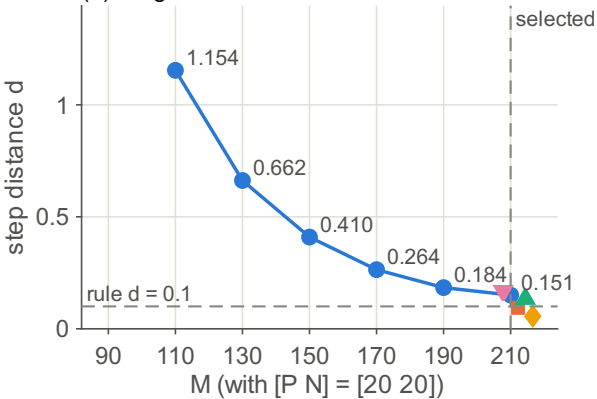
(a) Stage 0 truncation ladder
